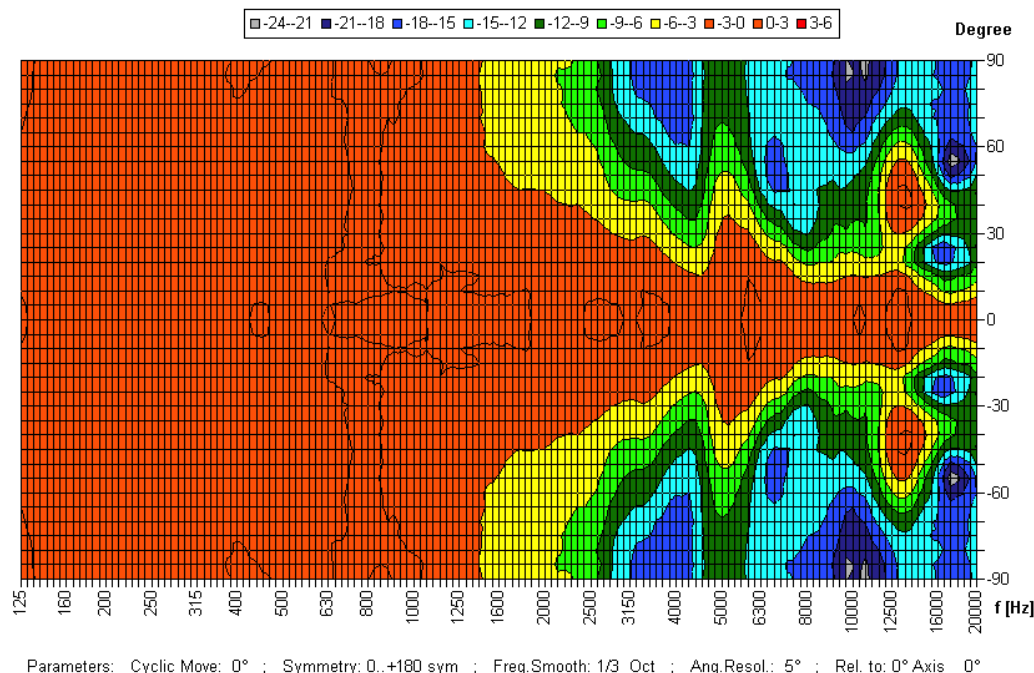
Horizontal Isobars of: Elko-Schmid DLS-180-DC
